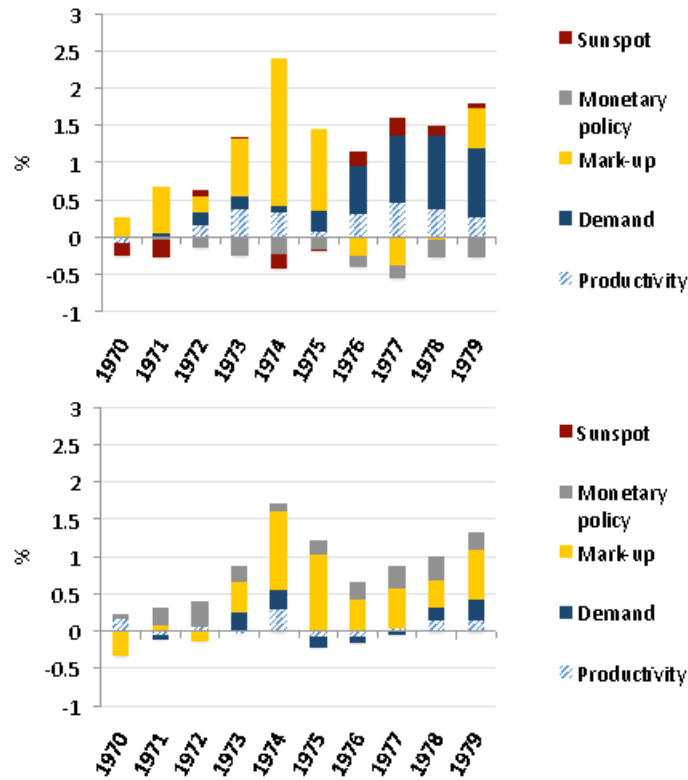
Figure 6: Sample 1970-1979. Historical decomposition of the deviation of the inflation rate from its steady state under indeterminacy (top) and determinacy (bottom) at quarterly rates.
