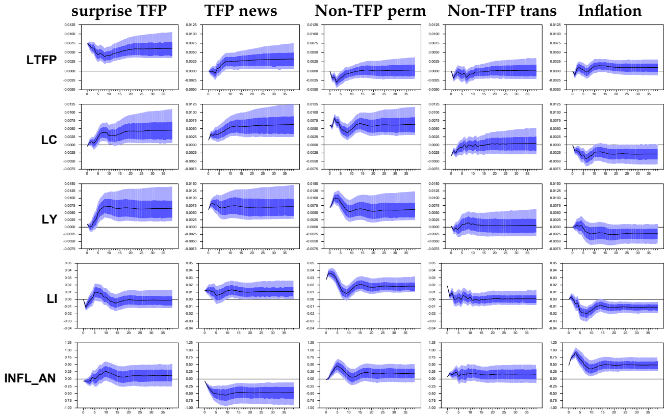
Figure B.3: Impulse response functions for the 5-variable VEC model with TFP (LTFP), consumption (LC), output (LY), investment (LI) and annualized inflation (INFL_AN), including 2 cointegrating relationships and 6 lags. Sample period is 1948-1979:01. The graph displays the variables responses (rows) to the five shocks: Column 1: surprise TFP, Column 2: TFP news, Column 3: non-TFP permanent, Column 4: non-TFP transitory, Column 5: Inflation. We obtain the Bayesian simulated distribution of IRF by Monte Carlo integration with 5000 replications. The black solid line represent the median response. We plot the distribution of IRF at 16% to 84% interval (dark blue) and at 5% to 95% interval (light blue)
