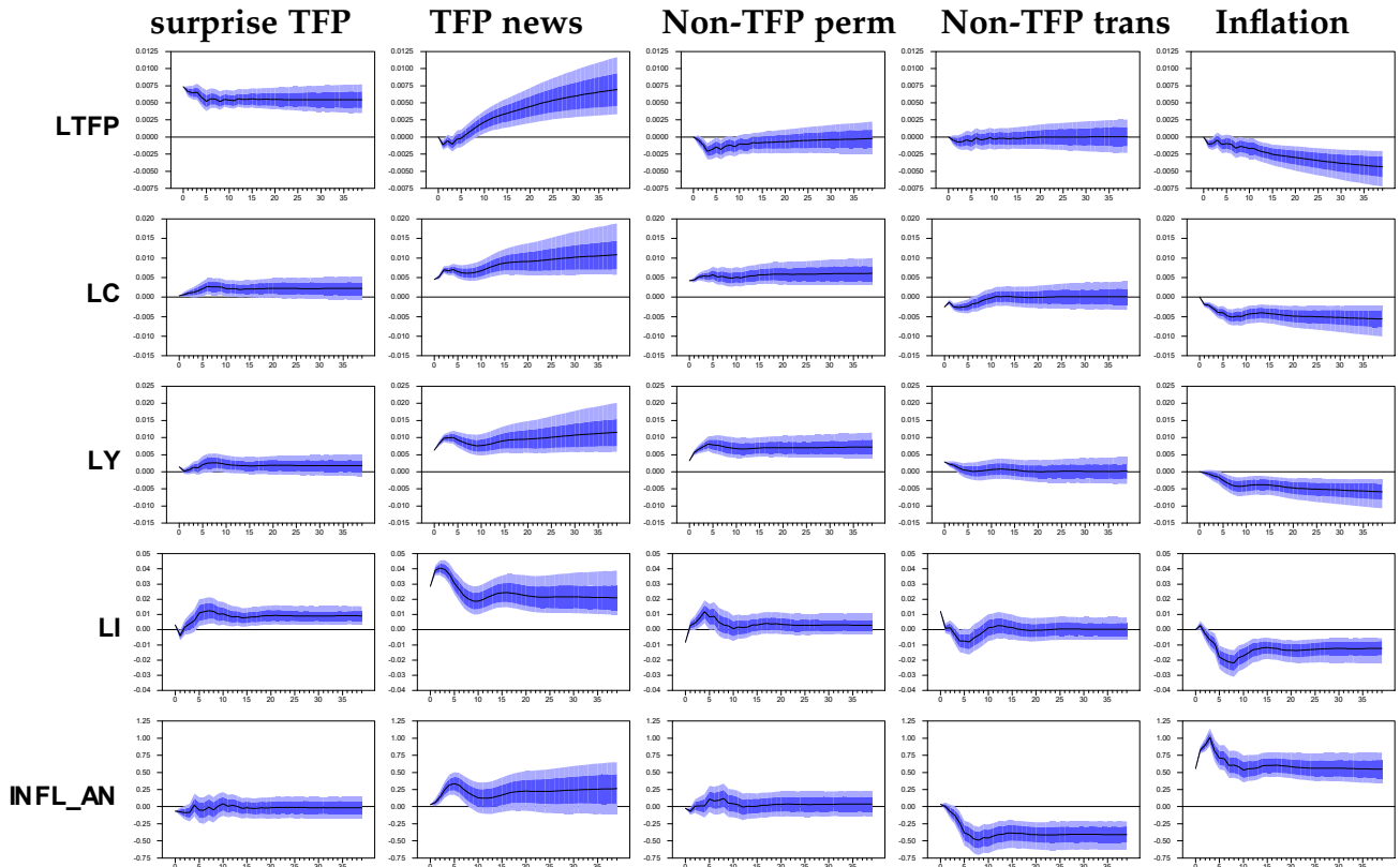
Figure 3: Impulse response functions for the 5-variable VEC model with TFP (LTFP), consumption (LC), output (LY), investment (LI) and annualized inflation(INFL_ AN), including 2 cointegrating relationships and 6 lags. Sample period is 1948-2017. The graph displays the variables responses (rows) to the five shocks: Column 1: surprise TFP, Column 2: TFP news, Column 3: non-TFP permanent, Column 4: non-TFP transitory, Column 5: Inflation. We obtain the Bayesian simulated distribution of IRF by Monte Carlo integration with 5000 replications. The black solid line represent the median response. We plot the distribution of IRF at 16% to 84% interval (dark blue) and at 5% to 95% interval (light blue)
