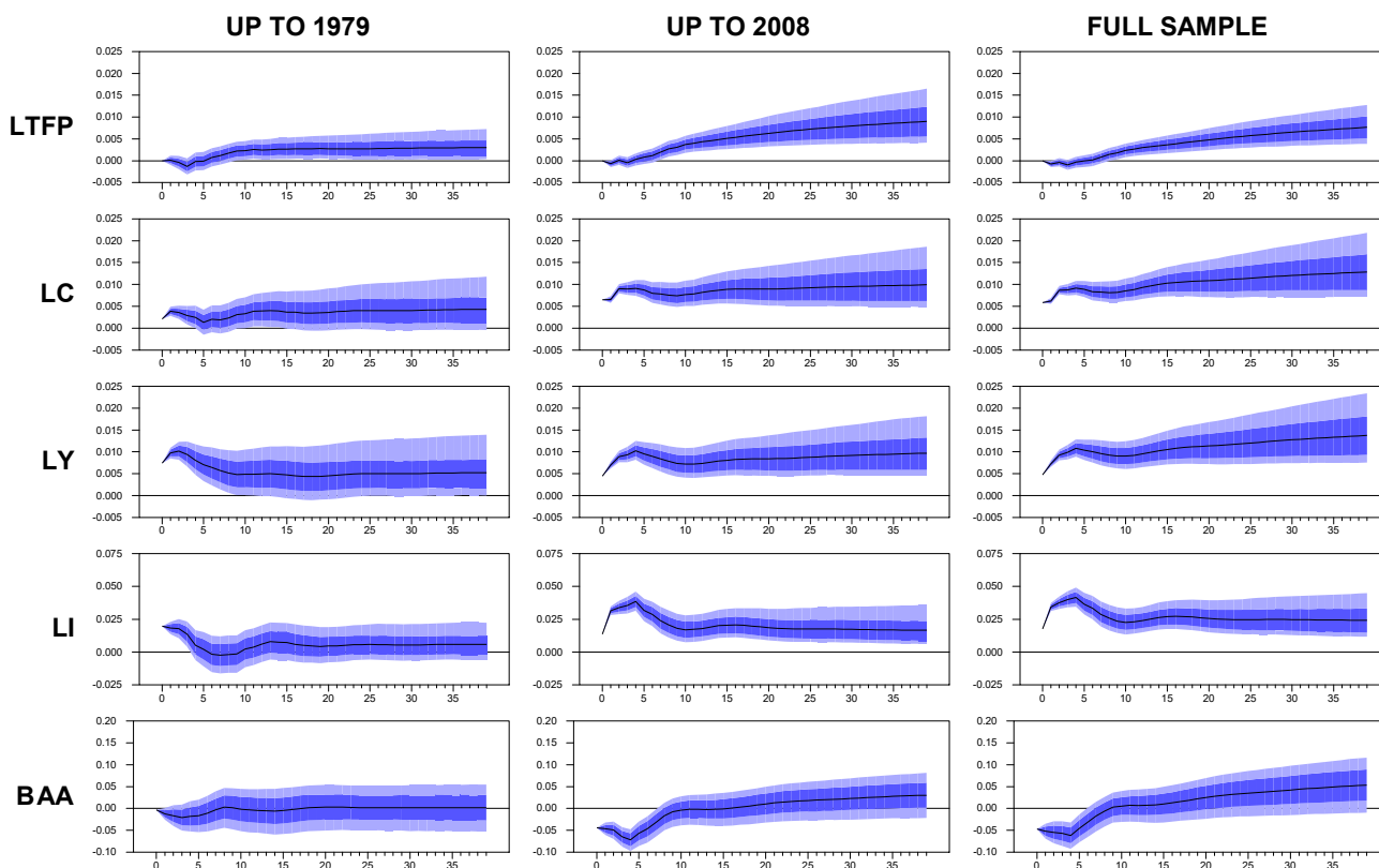
Figure 7: Impulse response functions for the 5-variable VEC model with TFP (LTFP), consumption (LC), output (LY), investment (LI) and Baa corporate spread (BAA), including 2 cointegrating relationships and 6 lags. In the rows we represent the variables and in the columns are the three different sample periods: 1948-1979q1, 1948-2008q3, 1948-2017q3. We obtain the Bayesian simulated distribution of IRF by Monte Carlo integration with 5000 replications. The black solid line represent the median response. We plot the distribution of IRF at 16% to 84% interval (dark blue) and at 5% to 95% interval (light blue)
