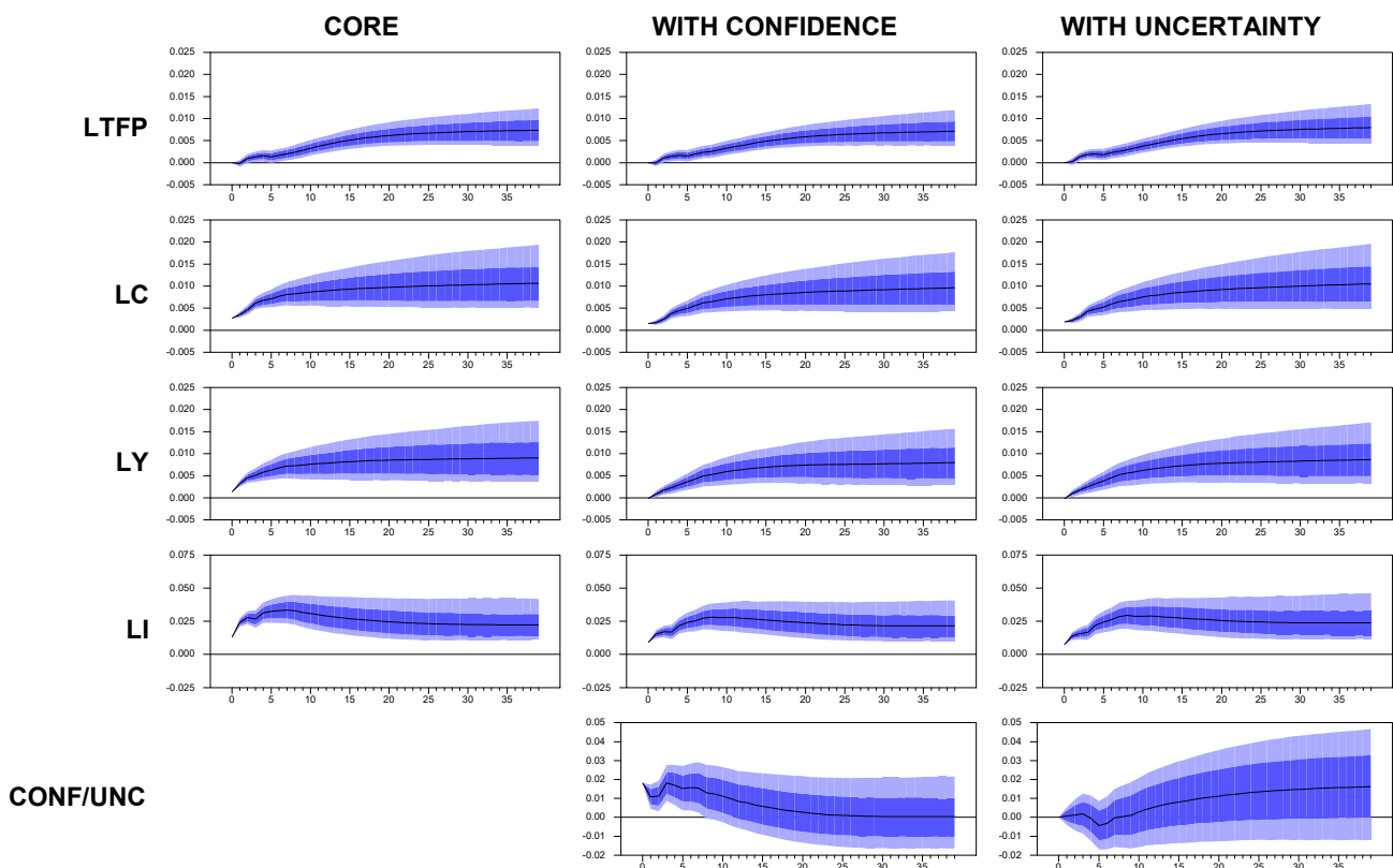
Figure 9: Impulse response functions after a technology news shock for three different structural VEC models for the period 1960q3-2017q3. Core (column 1): 4-variable VEC model with TFP (LTFP), consumption (LC), output (LY), investment (LI) and hours worked (LH), including 2 cointegrating relationships and 6 lags. Core sVECM extended with confidence (column 2). Core sVECM extended with uncertainty (column 3). Rows represent the variables. We obtain the Bayesian simulated distribution of IRF by Monte Carlo integration with 5000 replications. The black solid line represent the median response. We plot the distribution of IRF at 16% to 84% interval (dark blue) and at 5% to 95% interval (light blue)
